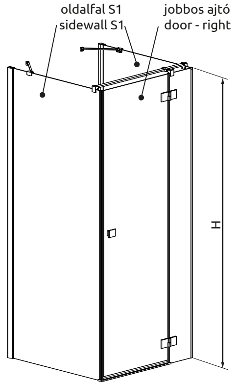
Jobbos kabin Variant R
